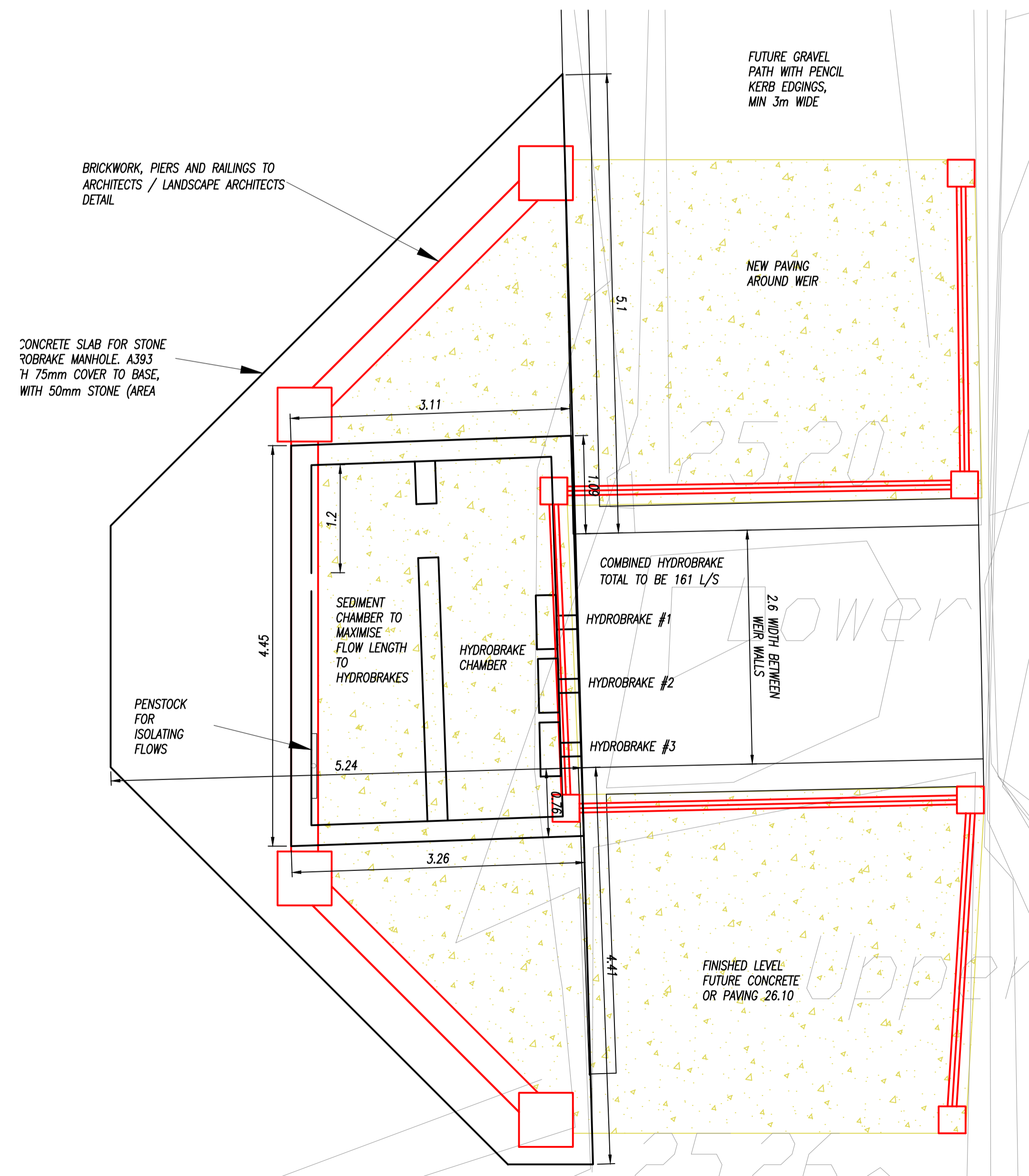
PLAN OF HYDROBRAKE MANHOLE / WEIR AREA
